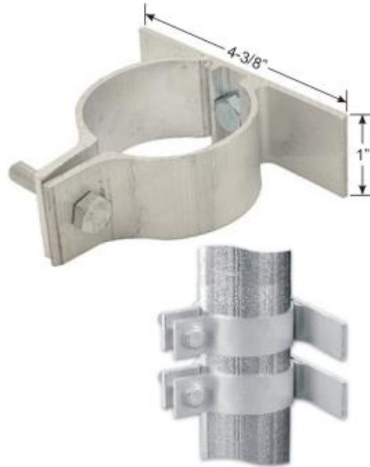
(Figure 1 PIPE POST BRACKETS)
